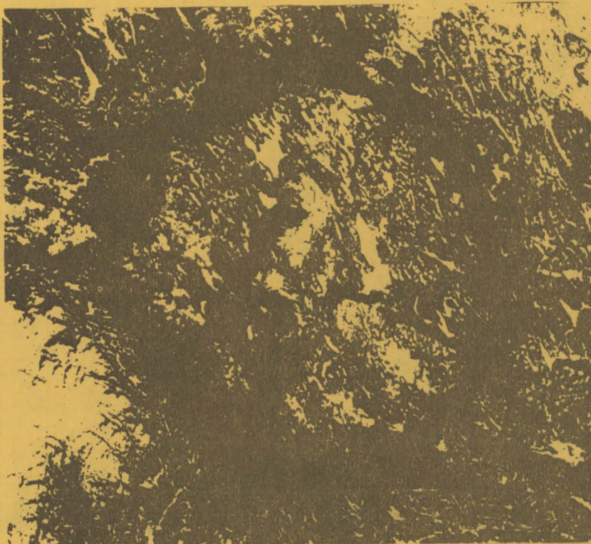
Bild. Manicouagan-kratern i Quebec. 70 km bred
